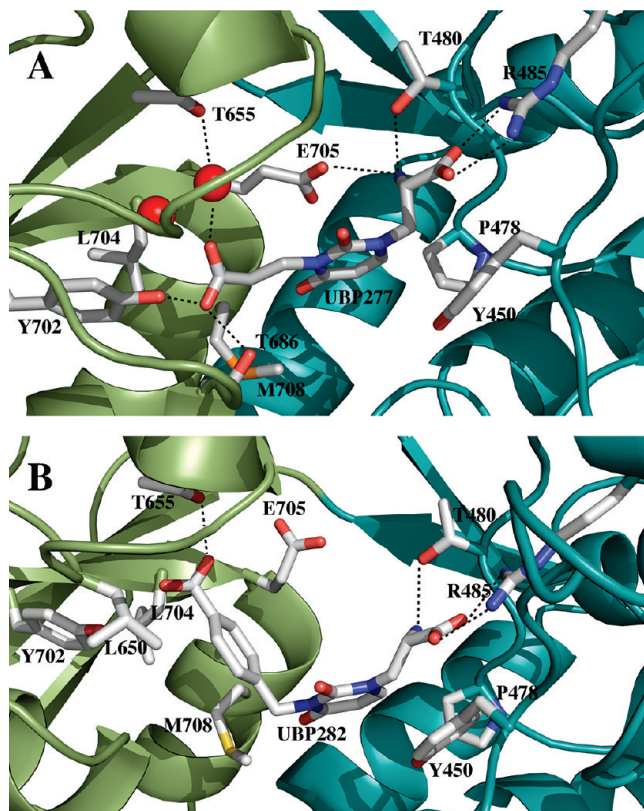
FIGURE 1: Structures of the binding sites for UBP277 (A) and UBP282 (B) on GluR2 S1S2. In each case, lobe 1 is shown in cyan and lobe 2 is in green. Interactions between the ligand and protein side chains are indicated. Additional interactions with the backbone are also made with lobe 1.
