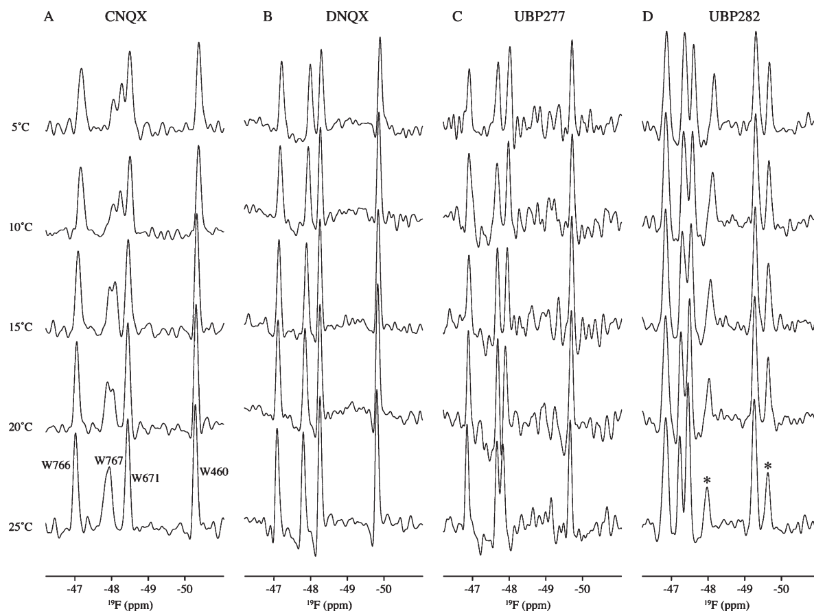
FIGURE 4: ^{19}\text{F} NMR spectra of antagonists bound to 5- ^{19}\text{F} -tryptophan-labeled GluR2 S1S2 as a function of temperature: (A) CNQX, (B) DNQX, (C) UBP277, and (D) UBP282. The signal for W767 is in chemical exchange for the CNQX-bound form but apparently not for S1S2 bound to the other three antagonists. Two additional peaks (marked with asterisks) were consistently seen in spectra of the UBP282-bound form and are consistent with chemical shifts observed in the apo form.
