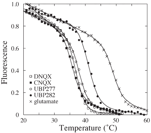
FIGURE 7: Thermal denaturation of GluR2-S1S2 bound to glutamate, CNQX, DNQX, UBP277, and UBP282. The temperature was increased at a rate of 0.06 min/ ^{\circ} C. The data were fit as described by Madden et al. (34).
