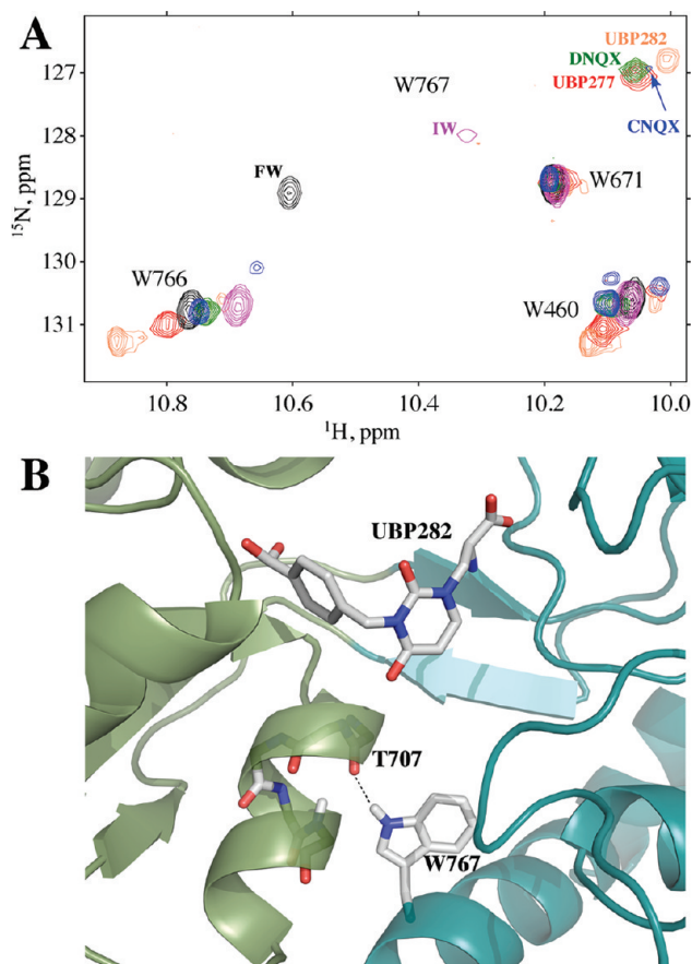
FIGURE 5: (A) A portion of the ^1\text{H} , ^{15}\text{N} -HSQC (TROSY) spectrum at 10 °C showing the side chain tryptophan amides for GluR2 S1S2 bound to a variety of willardiine agonists and antagonists as well as CNQX and DNQX. The signal for W767 varies with the orientation of the two lobes, moving upfield in both dimensions as the lobe opening increases. The amide proton makes a hydrogen bond across the lobe interface with the carbonyl of T707, shown here in the UBP277-S1S2 structure (B). The peak for this correlation is dramatically broadened at this temperature for IW and CNQX, but not the other compounds shown. This broadening is consistent with exchange between multiple relative orientations of the two lobes (10).
