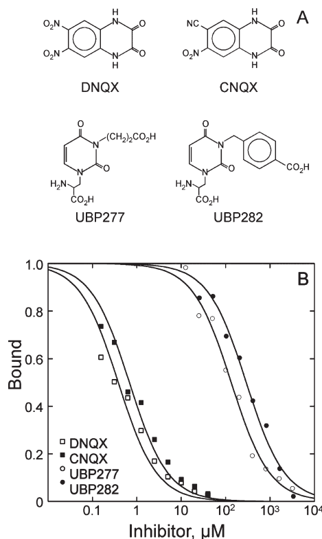
FIGURE 3: (A) Structures of the antagonists used in the binding study. (B) Inhibition of the binding of [^3\text{H}]\text{AMPA} to GluR2 S1S2 by DNQX, CNQX, UBP277, and UBP282. The \text{IC}_{50} values were 0.38 \pm 0.04 \mu\text{M} , 0.68 \pm 0.06 \mu\text{M} , 135 \pm 12 \mu\text{M} , and 292 \pm 26 \mu\text{M} , respectively.
