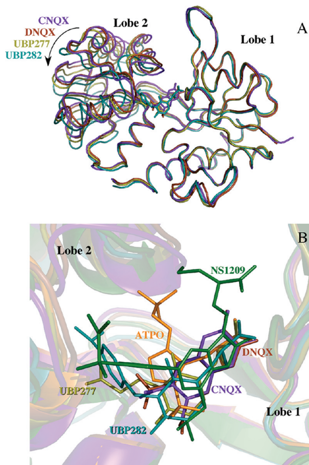
FIGURE 8: (A) Ribbon structures of GluR2-S1S2 bound to CNQX (purple, 3b7d; (17)), DNQX (brown, 1ftl; (15)), UBP277 (yellow), and UBP282 (cyan). The residues in lobe 1 are aligned to illustrate the different lobe orientations. Using DynDom (41), the lobe opening relative to the glutamate-bound form (1ftj, C protomer; (15)) is 15.7^\circ \pm 0.5^\circ for CNQX, 16.5^\circ \pm 1.1^\circ for DNQX, 19.8^\circ \pm 0.6^\circ for UBP277, and 26.7^\circ \pm 1.8^\circ for UBP282. (B) Overlay of the binding site for six antagonists showing the multiple sites of interaction. Shown are CNQX, DNQX, UBP277, UBP282 (as in part A), ATPO (orange, 1n0t; (16)), and NS1209 (green, 2cmo; (18)). As in part A, the residues in lobe 1 were aligned.
