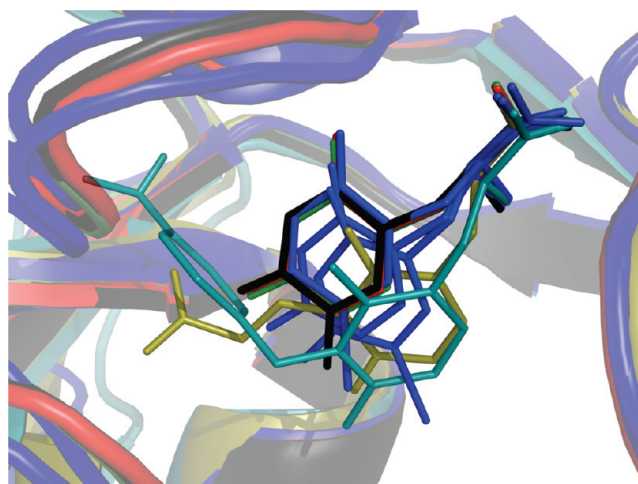
FIGURE 2: The orientation of different willardiines in the GluR2 S1S2 binding site is illustrated. The residues in lobe 1 were aligned. The positions of HW (red; 1mqj), BrW (green; 1mqh), and FW (black; 1mqi) are superimposable. However, the positions of IW (blue; 1mqg) varies within the same crystal. IW is the lowest efficacy of the four partial agonists. UBP277 (yellow) and UBP282 (cyan) move even further down the binding pocket than IW and make contact with lobe 2 through the substituents in the 2 position.
