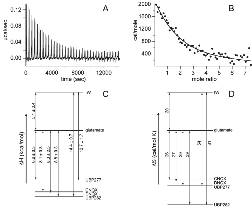
FIGURE 6: (A, B) Sample data from ITC competitive binding studies: 500 \mu M UBP277 titrated into 12 \mu M S1S2 bound to glutamate at 10 ^{\circ} C. The data were fit using Origin 7 and the equations described by Sigurskjold et al. (33) for competition binding. (C, D) Schematic of the relative enthalpies and entropies of binding of various ligands to S1S2 as determined by competitive binding ITC experiments.
